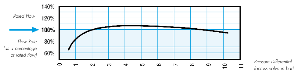
Performance Graph – Typical of all PRECISION valves irrespective of body size or flow rate
